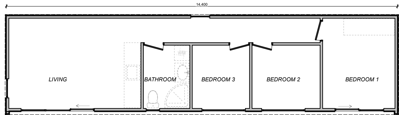
THREE BEDROOM 3.5 x 14.4, 14.8, 15.2m
