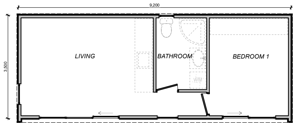
ONE BEDROOM 3.5 x 9.2, 9.6, 10.0m
