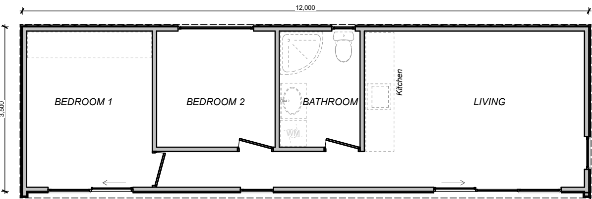
TWO BEDROOM 3.5 x 12.0, 12.4, 12.8m
